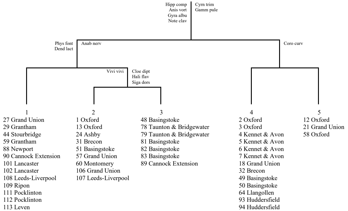
Figure 2.1. Revised TWINSpan classification of canal invertebrate assemblages using edge samples only
