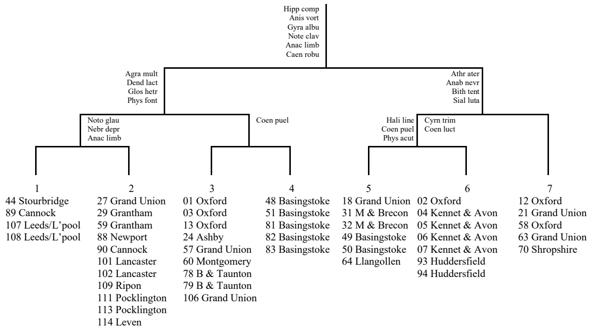
Figure 2.2. Original TWINSpan classification of canal invertebrate assemblages using combined edge and bottom samples
