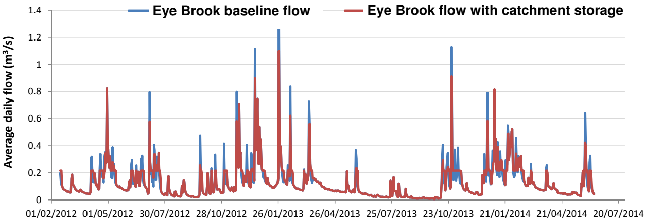
Figure 62. (a) Measured flow for the Eye Brook catchment and impact on flow of installing 37,500 m 3 of in-catchment water storage; data are expressed at a daily resolution as this is considered most relevant to downstream impacts on flood potential.
