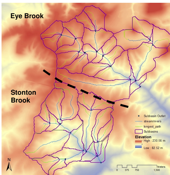
Figure 57. GIS project of the sub-basins and surface water network within the SWAT model projected onto a digital elevation model
