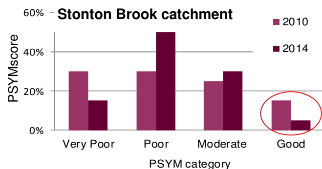
Figure 21. Pond quality trends in the three catchment areas between 2010 and 2014
