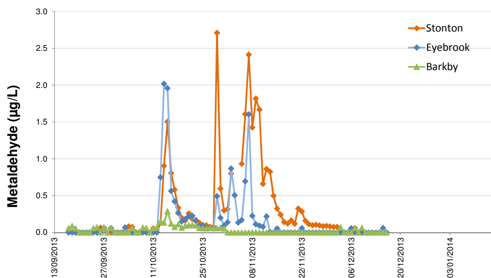
Figure 47. Metaldehyde runoff in winter 2013/14. (a) Barkby Brook, (b) Eye Brook, (c) Stonton Brook and (d) combined to show similarity of trends in the two catchments
