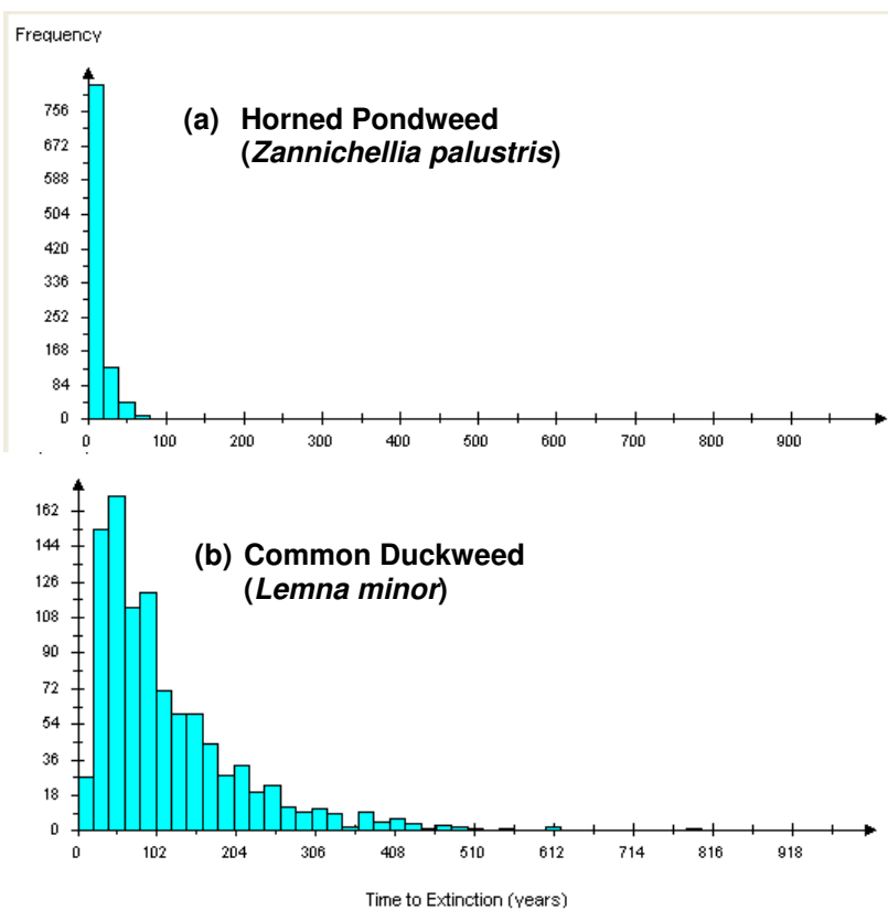
Figure 67. Time to extinction of (a) Horned Pondweed ( Zannichellia palustris ) and (b) Common Duckweed ( Lemna minor ) in the present 20 pond landscape of the Stonton Brook simulated using the Meta-X model.
