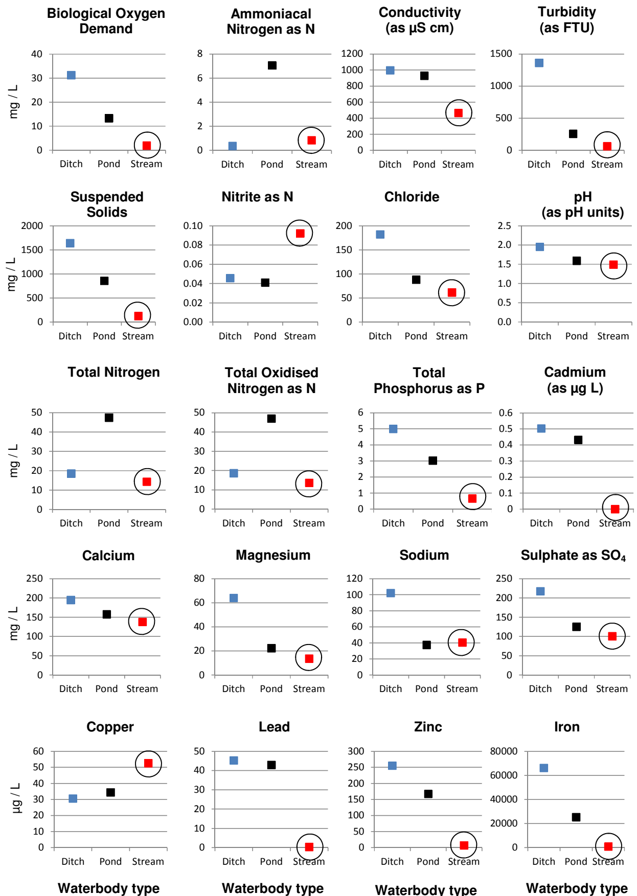
Figure 39. Chemical variability of freshwater habitats (ponds, ditches and streams) at the landscape scale. Graphs show range from minimum to maximum values for each determinand in the three waterbody types present in the Water Friendly Farming Landscape: ponds, ditches and streams. Data from all three catchment combined; n=60 for each habitat in all figures. Values are mg/L, unless stated in caption above graph, except metals which are µg/L. Streams are circled for clarity.
