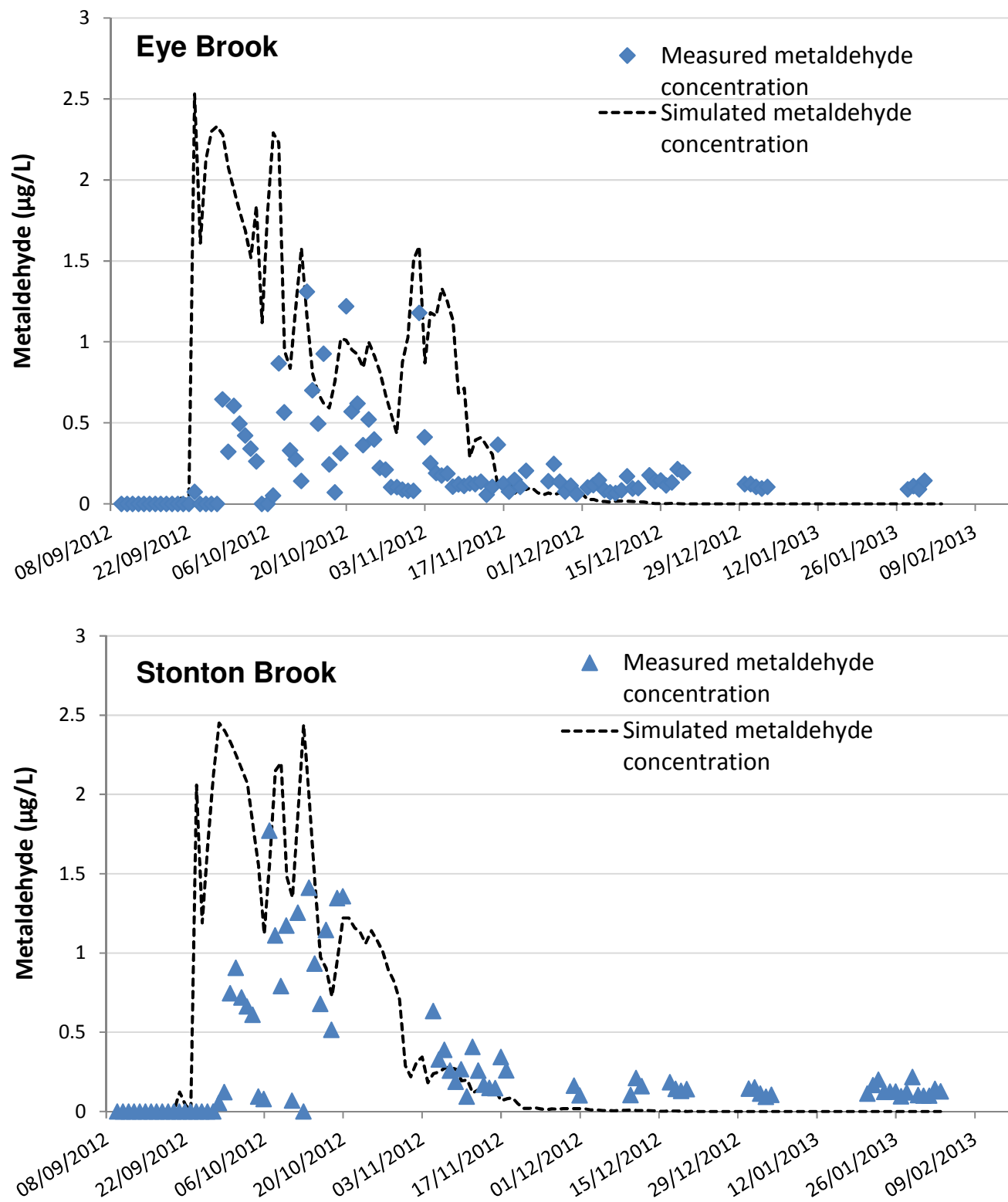
Figure 59. Comparison between observed concentrations of metaldehyde at the catchment outlets of Stonton Brook and Eye Brook and concentrations predicted by SWAT.
