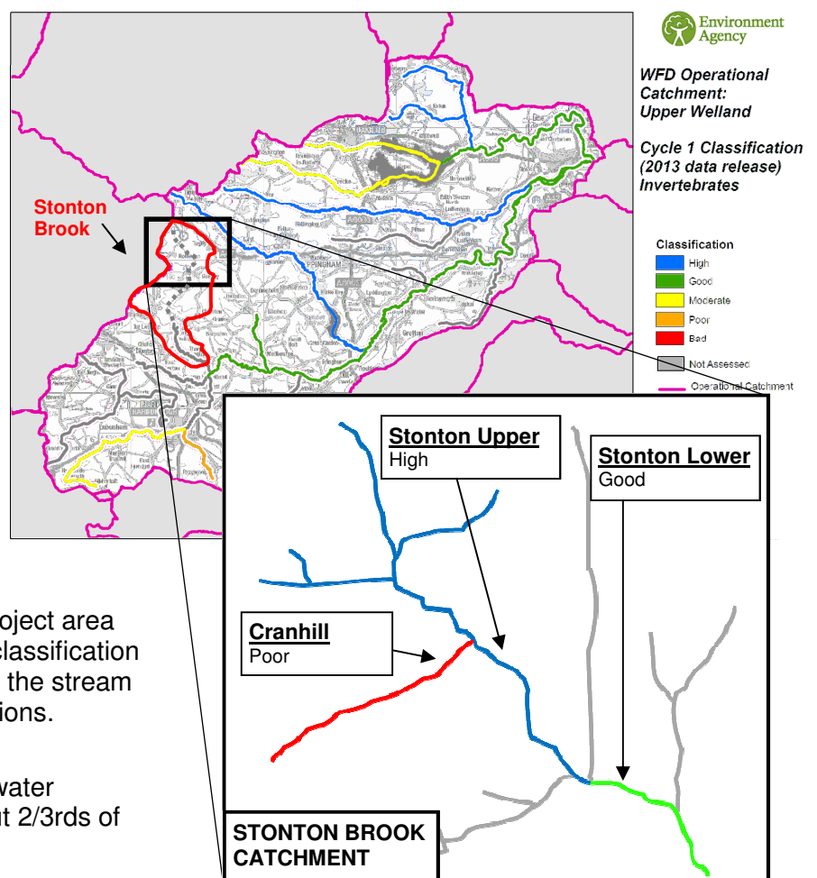
Figure 31. Water Framework Directive classification of tributaries in the Stonton Brook project area based on aquatic invertebrates. Different branches of the stream network vary from Poor to High status within the project area.
